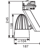
4-pin track adaptor
